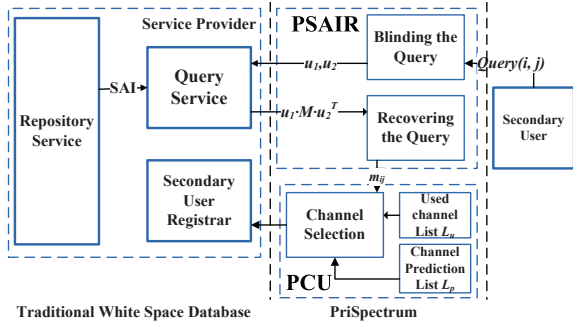
Fig. 4. Overview of PriSpectrum
