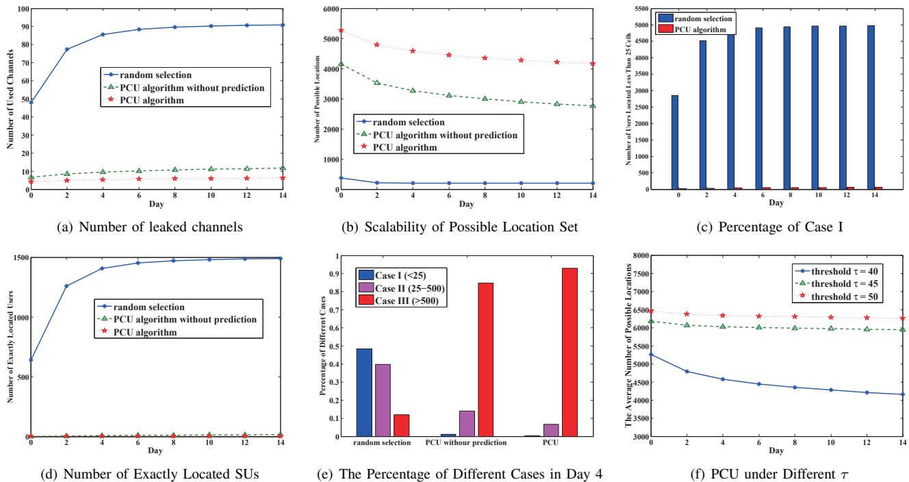
Fig. 6. Evaluation of Private Channel Utilization with Different Metrics
