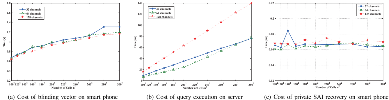
Fig. 5. Evaluation of Private Spectrum Query Module with Different Metrics
