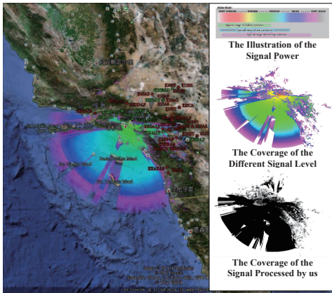
Fig. 2. The coverage of KRCA located at 118.062291^\circ , 34.213338^\circ with a 1707.0 m TV tower, whose channel is ch35 and ERP is 1000.000 kW
